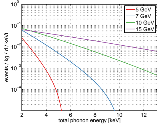
(b) Spectrum per total phonon energy (T2Z1 charge model)
